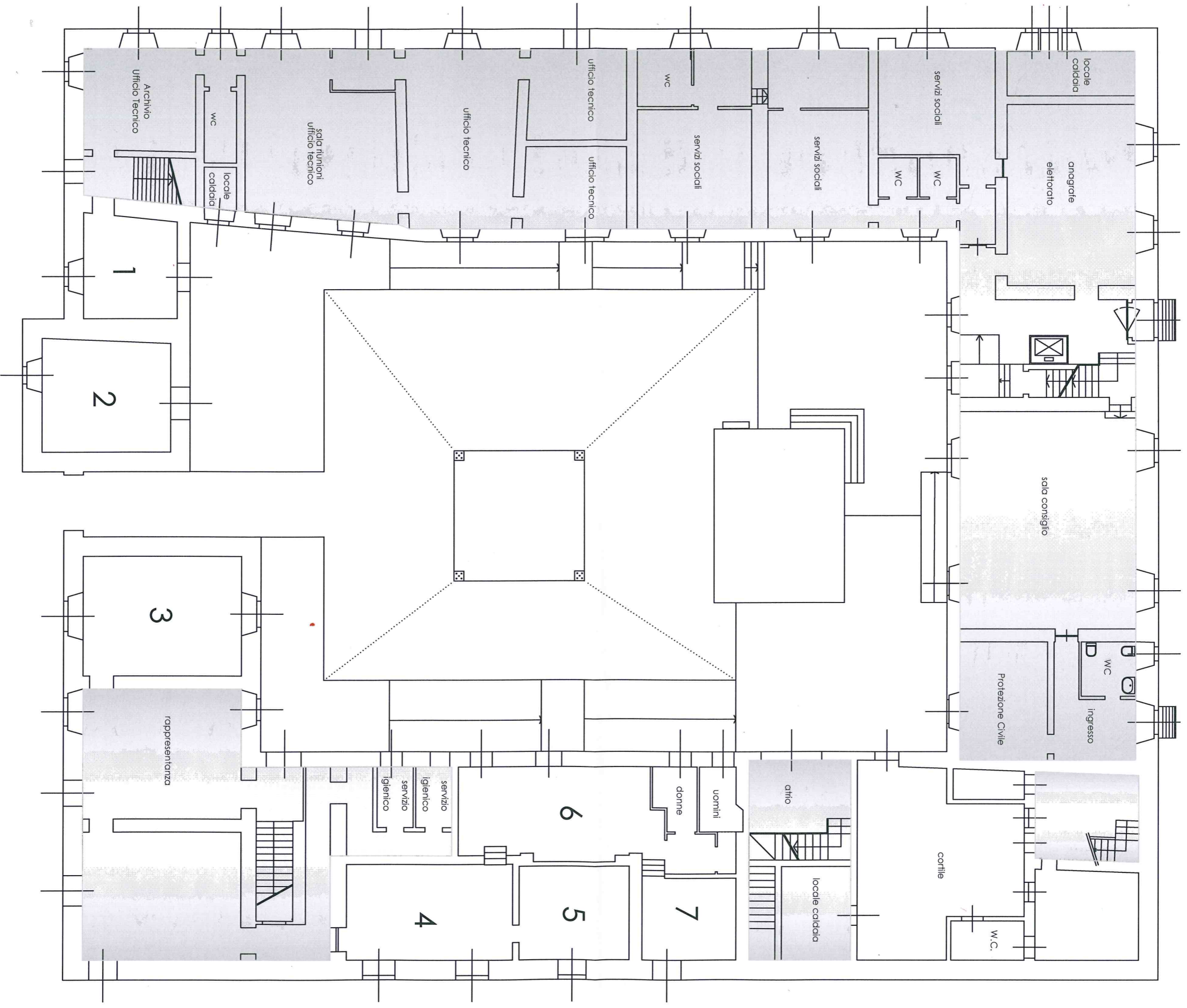
PIANO TERRA
